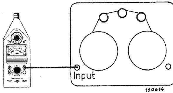
Fig. 9.4. The sound Level Meter used with a tape recorder.
