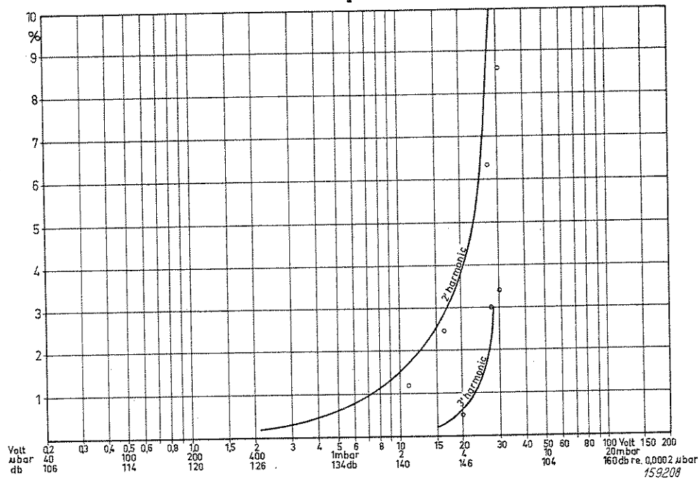
Fig. 5.9. Typical distortion curves for the one-inch microphones. The curves in full are measured on the cathode follower and referred to a complete microphone with a sensitivity of 5 \text{ mV}/\mu\text{bar} . The measuring points shown are averages measured in a pistonphone on a number of complete microphones at 50 Hz (c/s).
